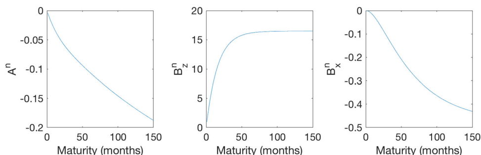
Figure 4. Model solution. This figure shows A^n , B_z^n , and B_x^n in the estimated model as defined by (20), (21), and (22) as functions of the maturity of dividends ( n ). (Color figure can be viewed at wileyonlinelibrary.com )
